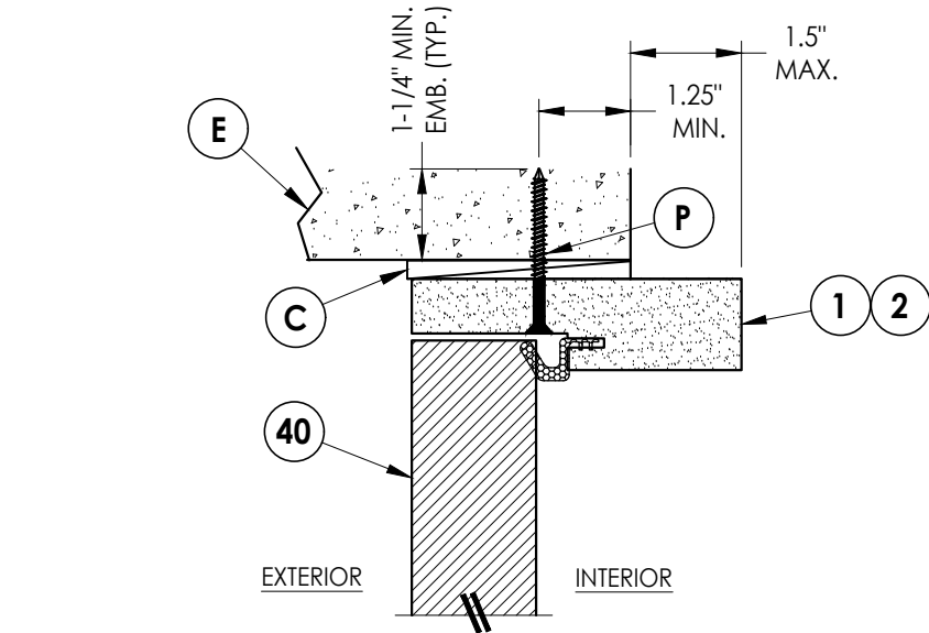
4 8 VERTICAL CROSS SECTION Shown Direct to Masonry Outswing only w/ 4-9/16" jamb Double Door Only (N/A w/ Sidelites)
