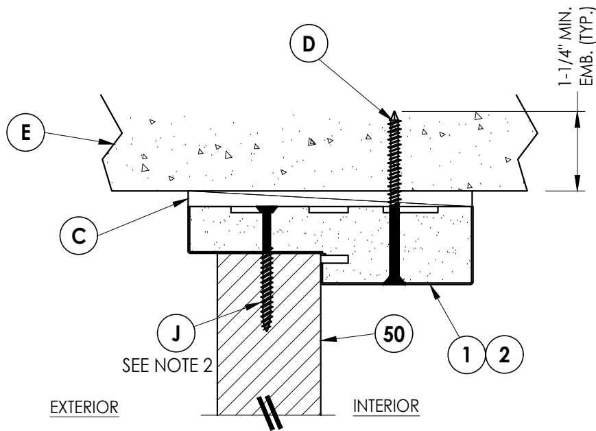
4 6 VERTICAL CROSS SECTION Shown Direct to Masonry Outswing shown (Inswing similar)
